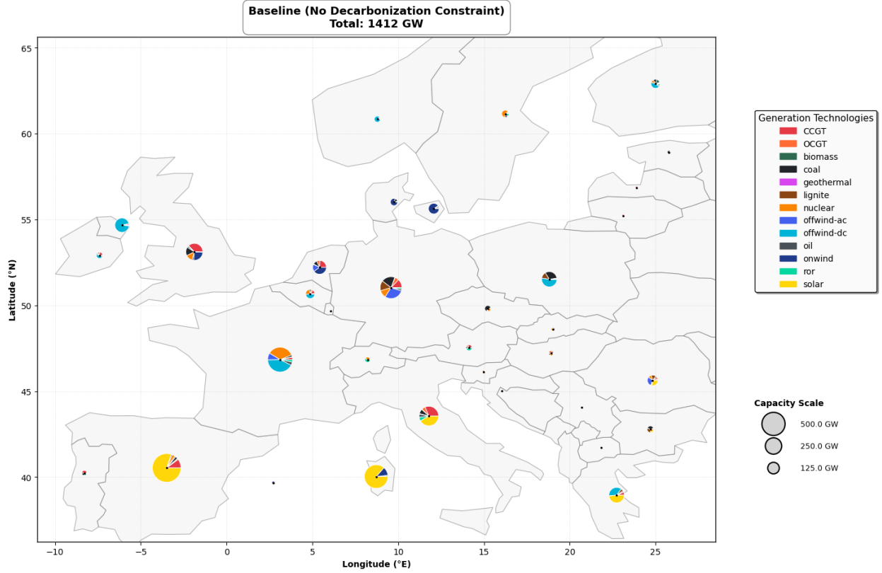
Figure 5: Baseline generator capacity map, showing installed generation capacity by technology and node.
