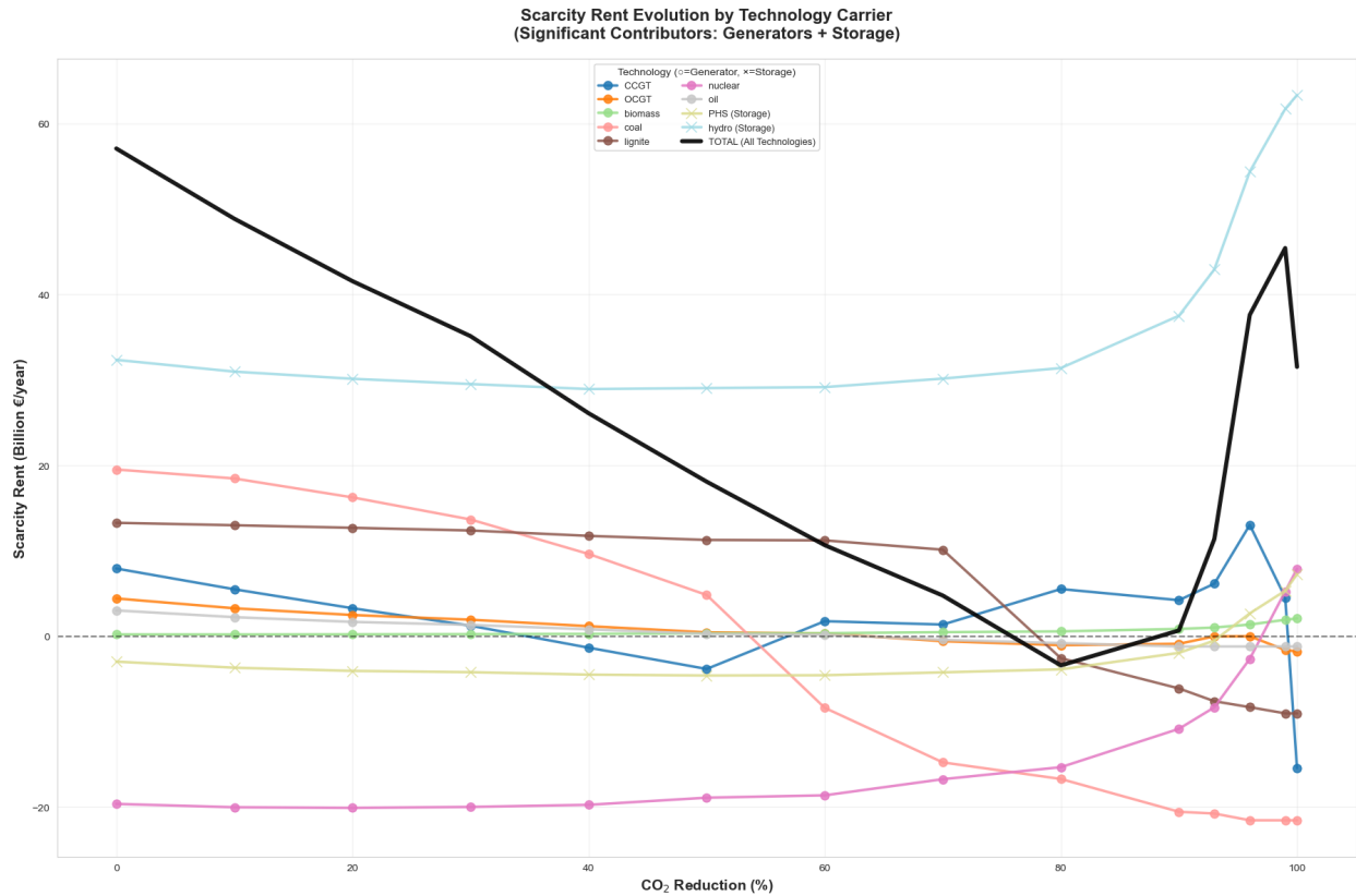
Figure 18: Scarcity rent contributions by technology shown as line chart by technology and level of decarbonization.
