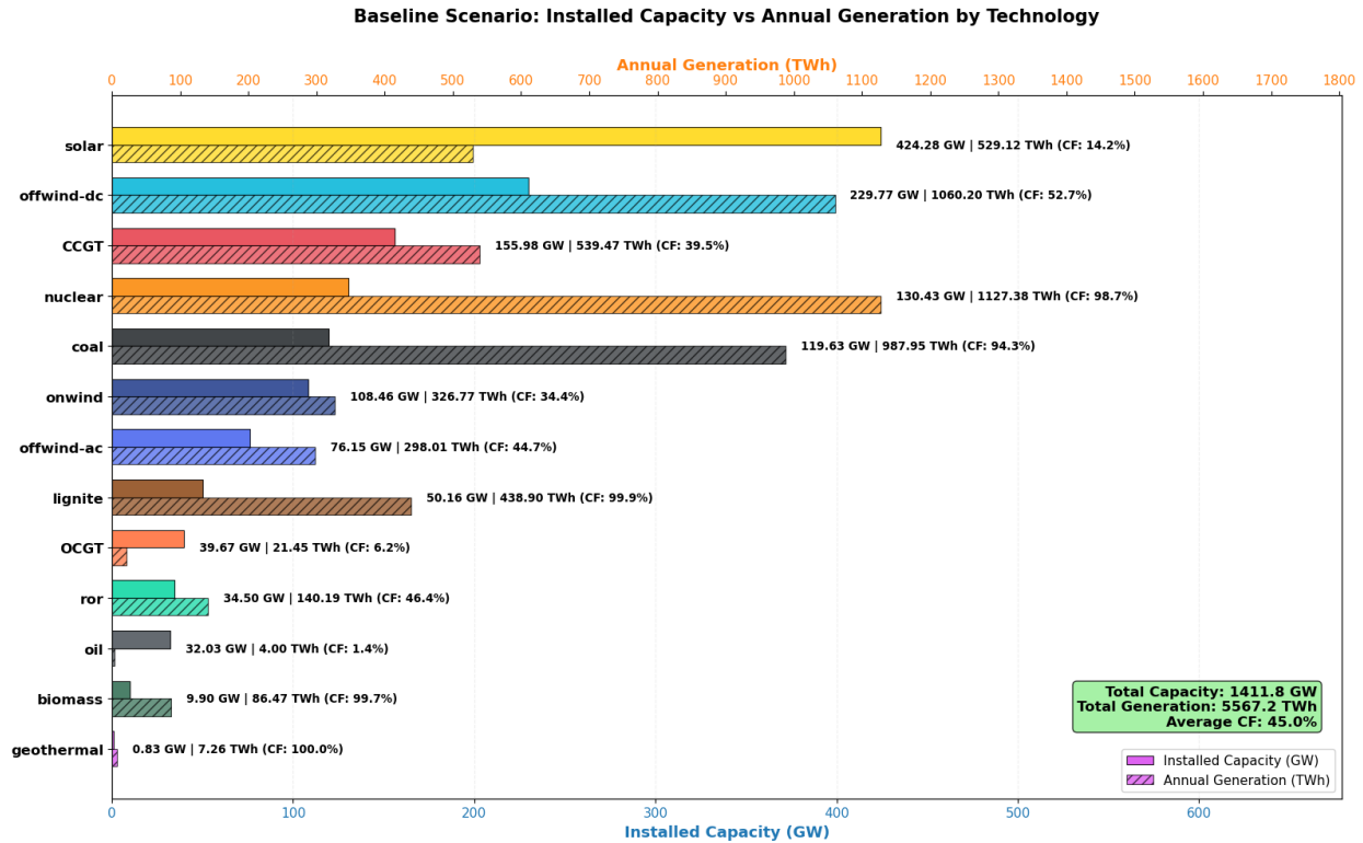
Figure 6: Baseline generator capacity and annual generation by technology, showing annual generation hatched and installed capacity solid.
