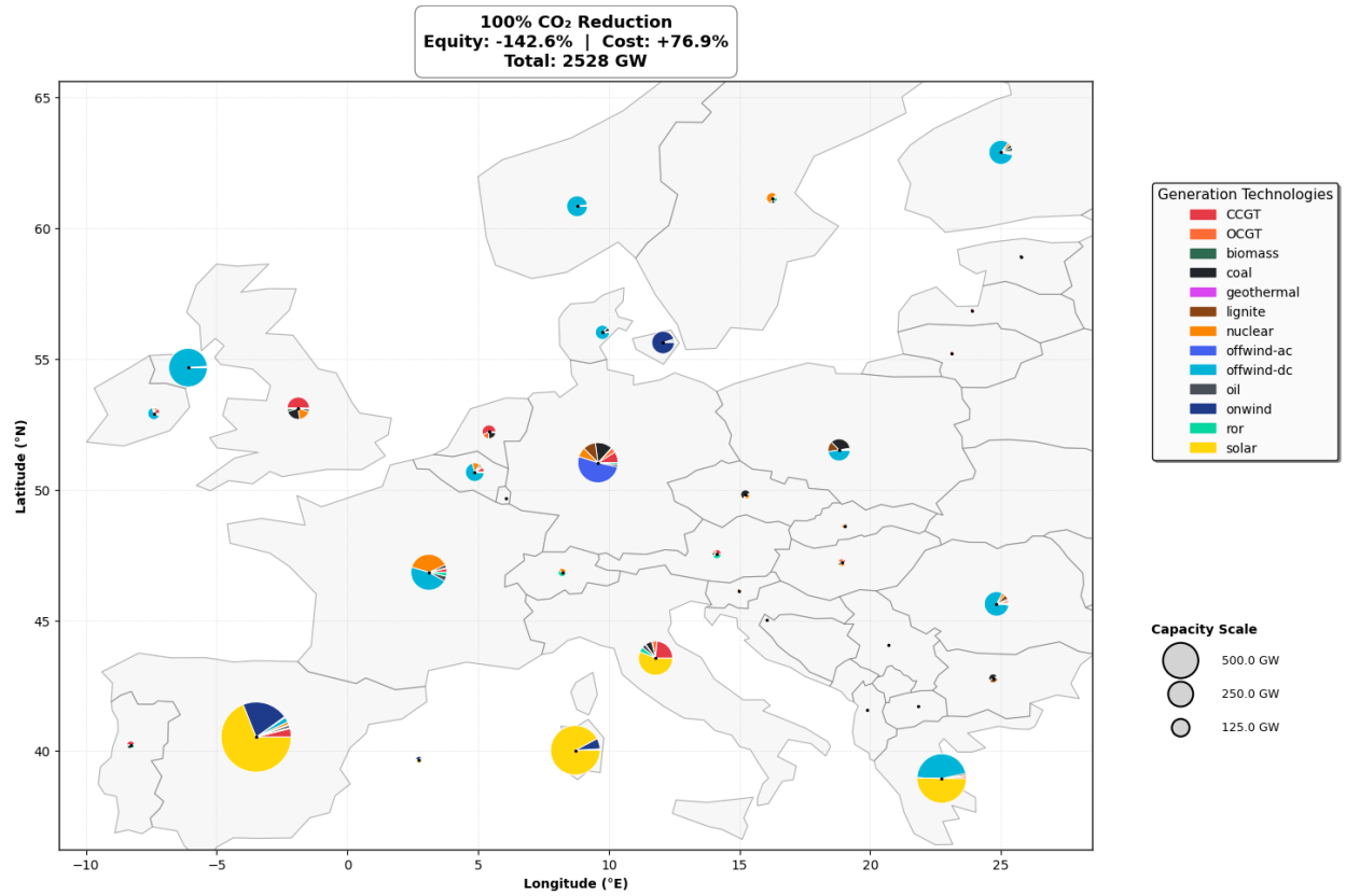
Figure 25: Generation capacity map at 100% decarbonization with pie charts showing generation mix by node.
