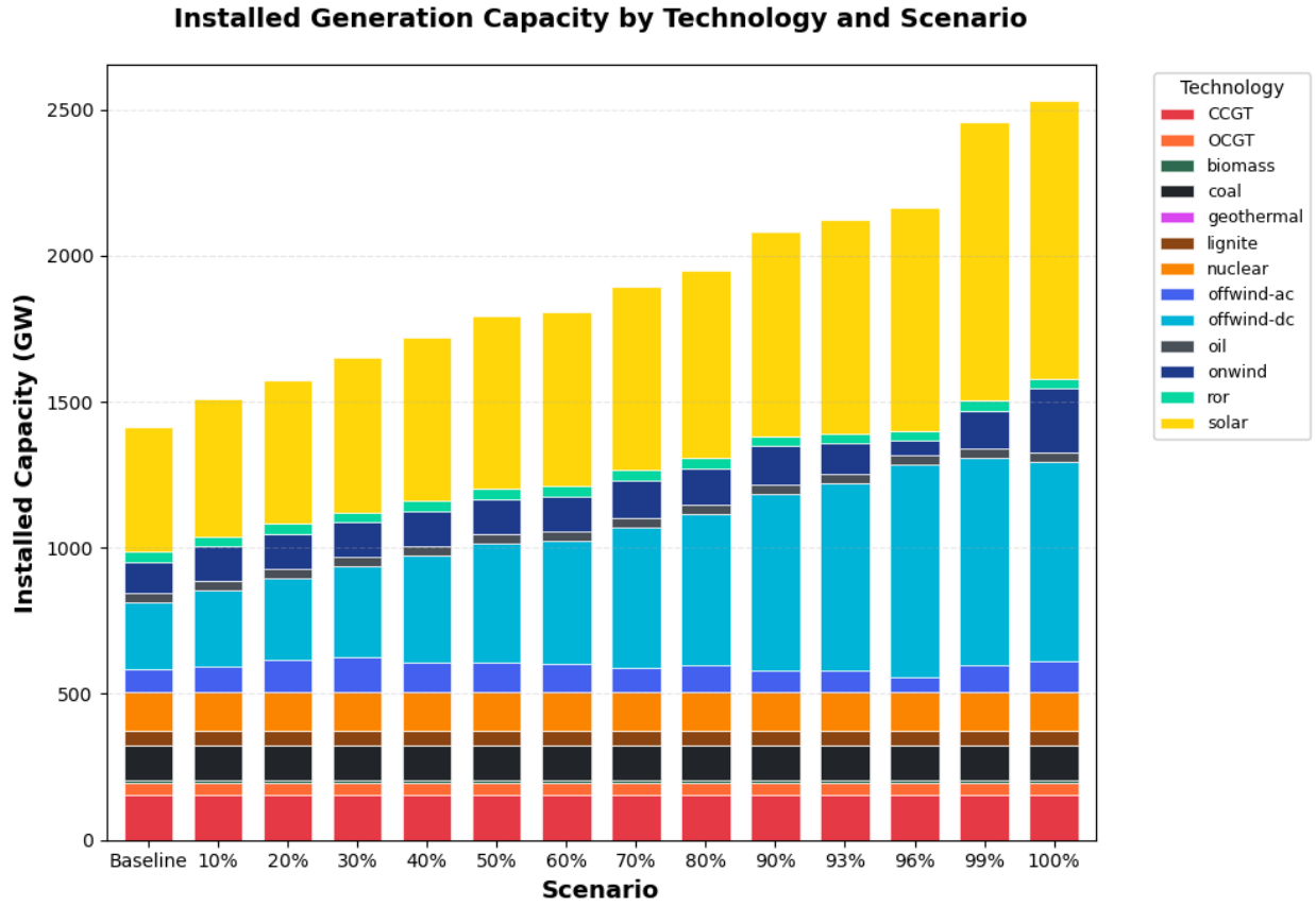
Figure 11: Decarbonized generator capacity by technology as bar chart by level of decarbonization.
