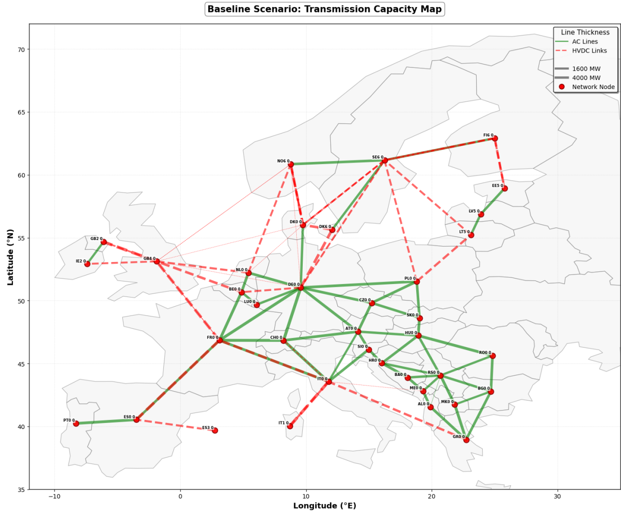
Figure 7: Baseline transmission capacity map, showing installed transmission capacity by AC lines and HVDC links.
