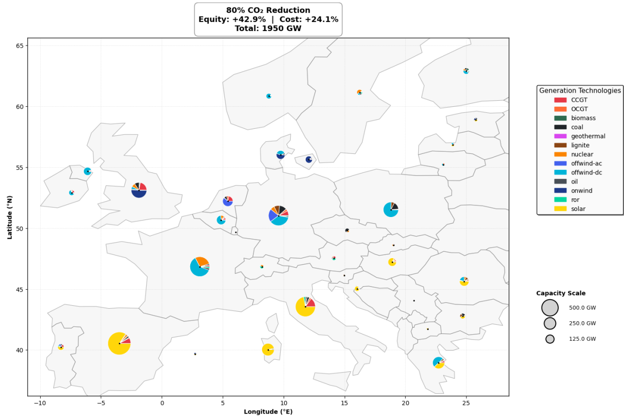
Figure 24: Generation capacity map at 80% decarbonization, with pie charts showing generation mix by node.
