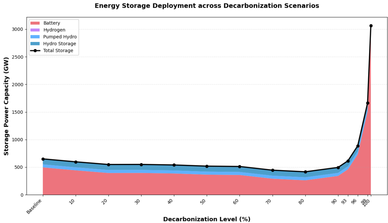
Figure 15: Decarbonized storage capacity by technology as stacked line plot
