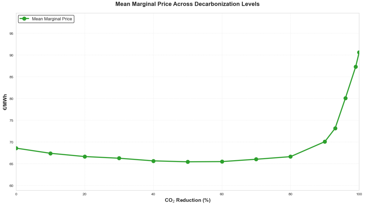
Figure 16: Decarbonized system mean marginal price as line plot by level of decarbonization.
