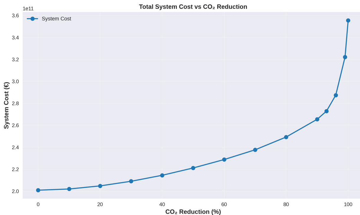
Figure 20: Total system cost in least-cost systems by level of decarbonization.
