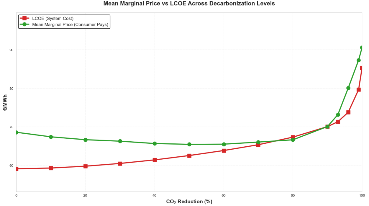
Figure 17: Comparison of mean LCOE and mean marginal price
