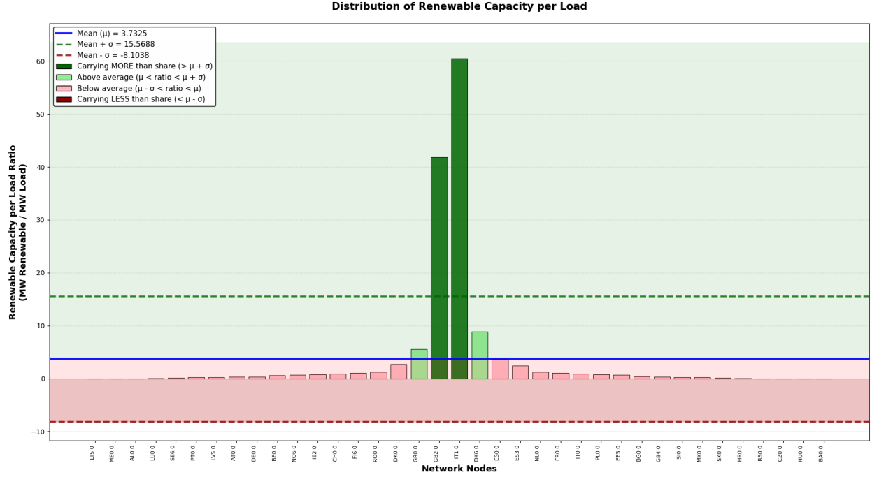
Figure 10: Baseline renewable capacity per load distribution with standard deviation bounds.
