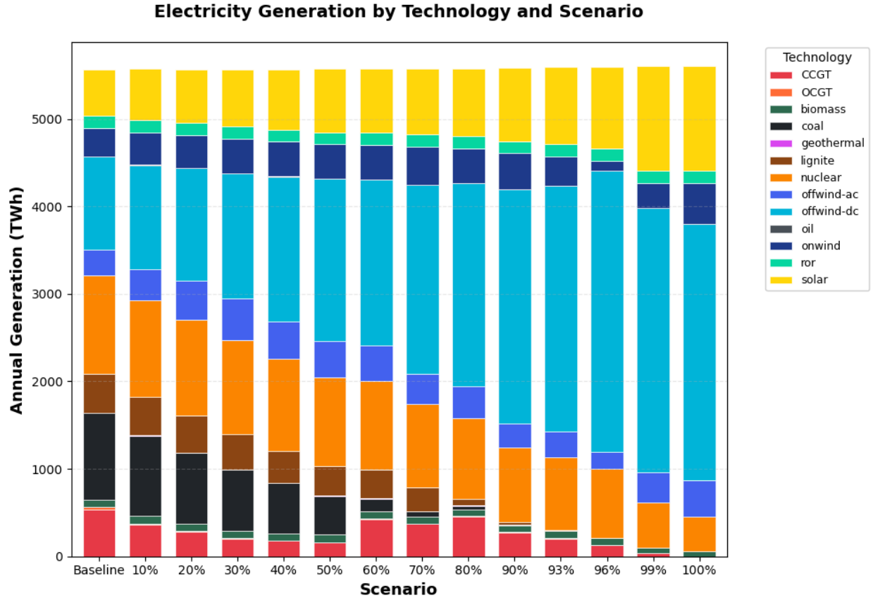
Figure 12: Decarbonized generator output by technology as bar chart by level of decarbonization.
