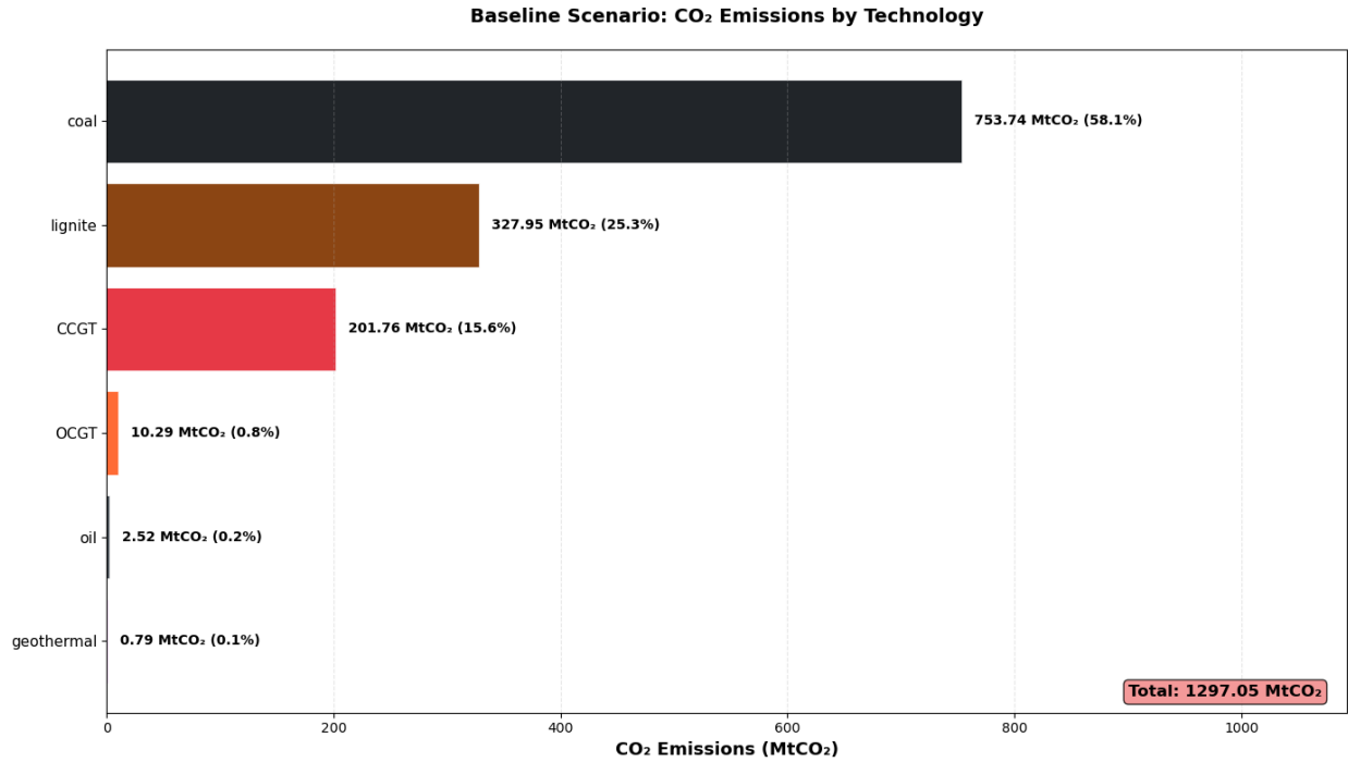
Figure 9: Baseline emissions by technology in MtCO_2 .
